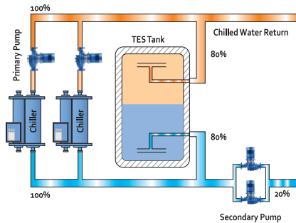
TES Charging (With Load)
