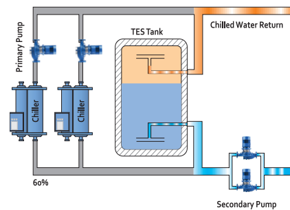
TES Discharging (With Chiller)
