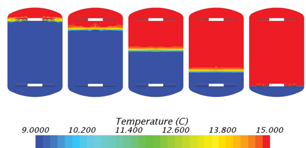
CFD Modelling – Discharging
