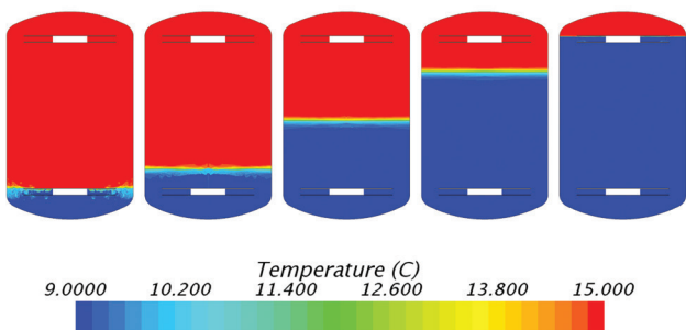
CFD Modelling – Charging
