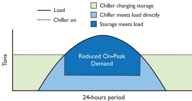
Source:ASHRAE Design Guide for Cool Thermal Storage Figure 3: Partial-Storage Demand-Limiting Operating Strategy
