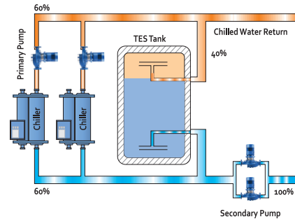
TES Discharging (With Chiller)
