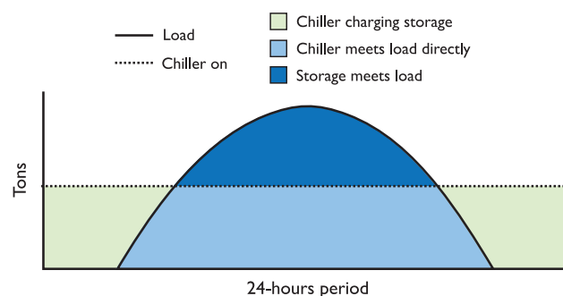
Figure 2: Partial-Storage Load-Levelling Operating Strategy
