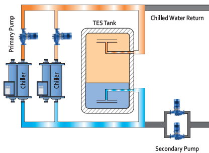
TES Charging (With Load)
